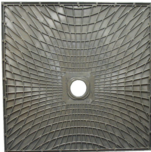
Underside of base showing arched structural ribbing and drain hole reinforcement ring.
